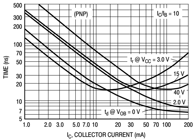
Figure 24. Turn-On Time
